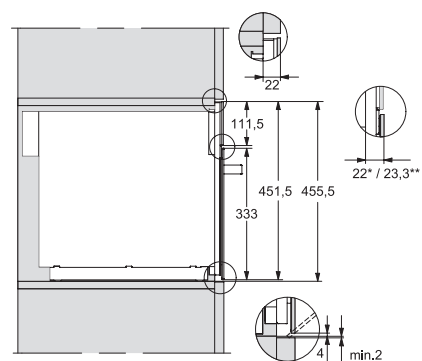
M7140TC, M724xTC, installation drawing
