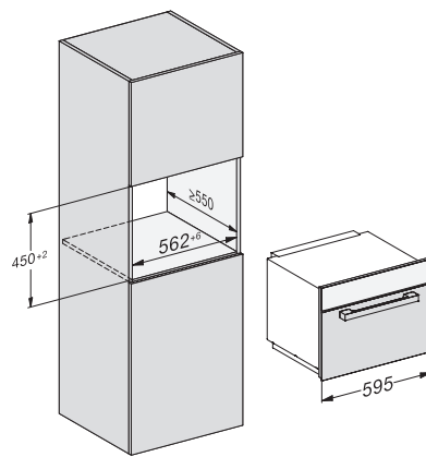
M7140TC, M724x, installation drawings
