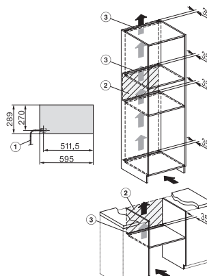
Installation ESW7x20, installation drawing
